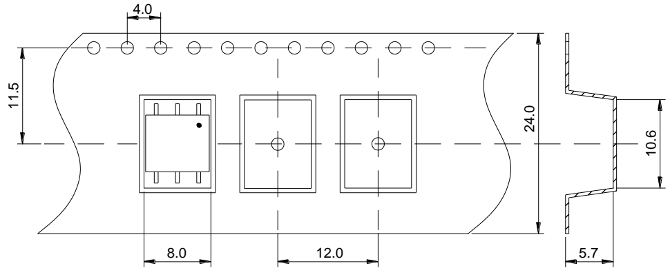
Tape & Reel
