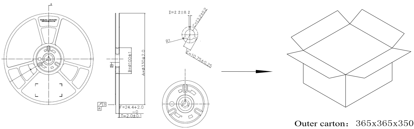
Tape & Reel
