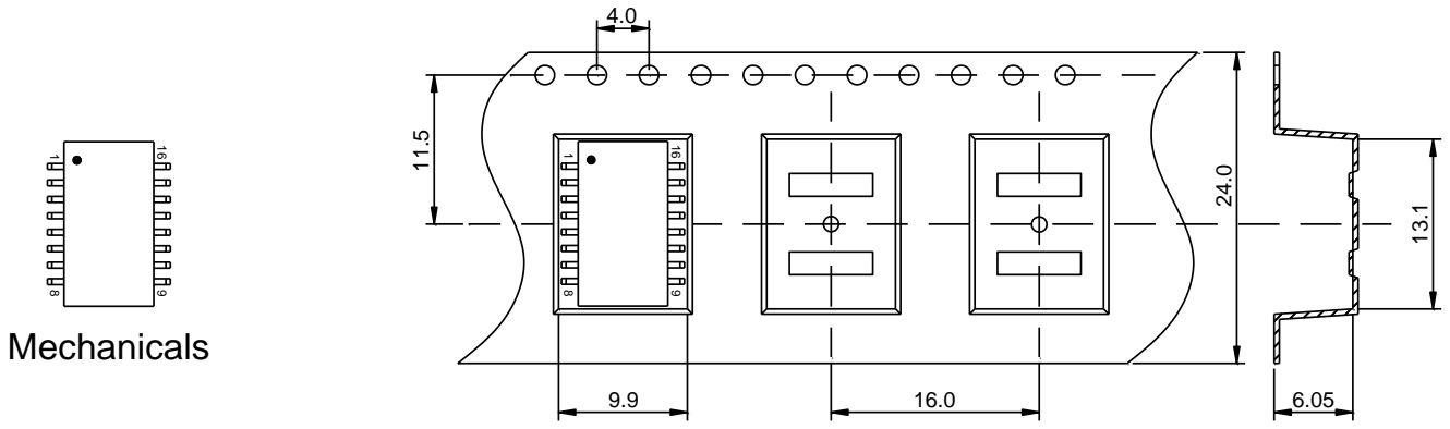
Tape & Reel
